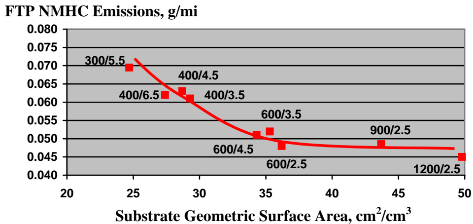
Figure 7. NMHC FTP emissions vs. substrate geometric surface area [see (15) for details]
