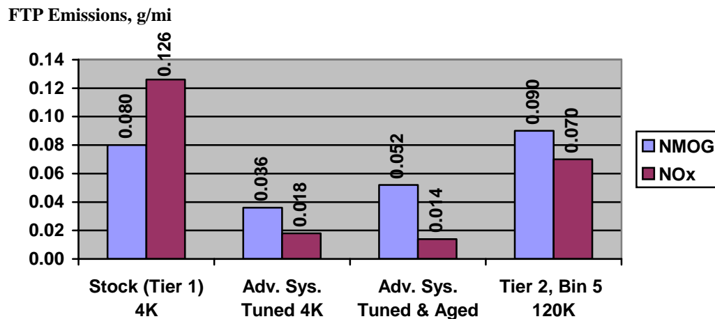
Figure 13. FTP emission performance of a 1997 Toyota T-100 light-duty truck equipped with an advanced emission control system
