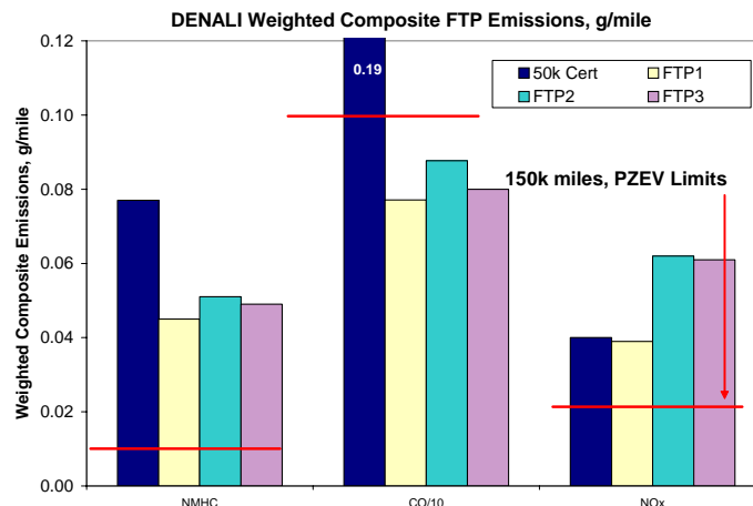
Figure 16. Weighted FTP Stock, Baseline Emissions – Denali
