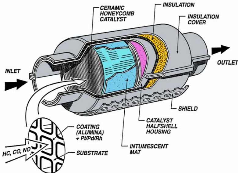
Figure 1. Three-way catalytic converter with ceramic substrates
