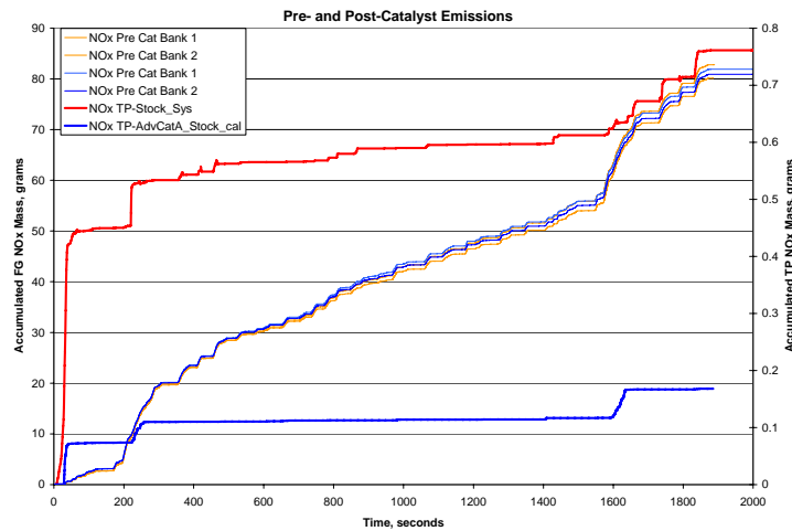
Figure 19. Modal NOx Emissions for the Denali Stock and Advanced System, both with the Stock Vehicle Calibration
