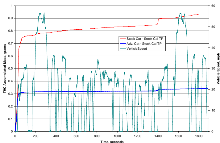
Figure 18. Accumulated THC Mass Emissions for the Denali Stock and Advanced System, both with the Stock Vehicle Calibration
