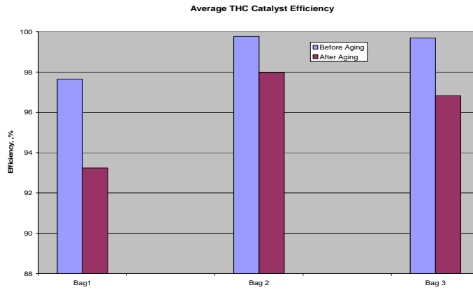
Figure 20. Denali THC Catalyst Efficiency Comparison Before and After Advanced System Aging
