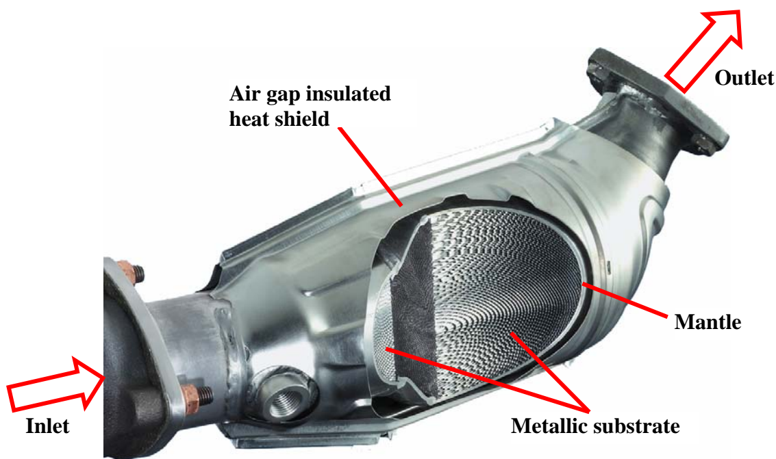
Figure 2. Three-way catalytic converter with metallic substrates
