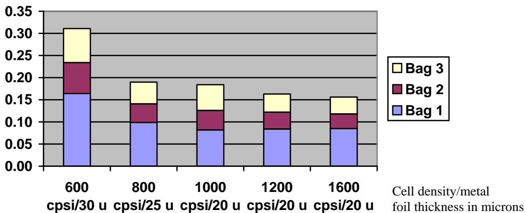
Figure 8. Accumulated FTP HC emissions for a three-way catalyst coated on high cell density metal substrates [see (27) for details]
