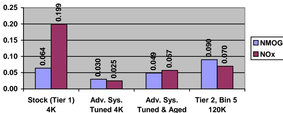
Figure 12. FTP emission performance of a 1997 Ford Crown Victoria equipped with an advanced emission control system
