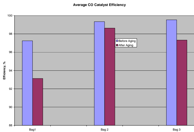
Figure 21. Denali CO Catalyst Efficiency Comparison Before and After Advanced System Aging
