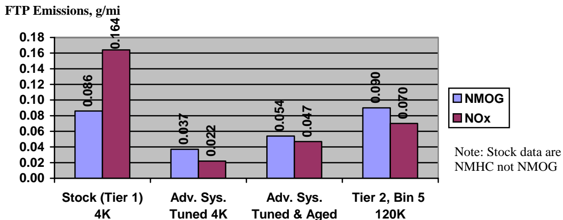
Figure 14. FTP emission performance of a 1999 Chevrolet Silverado light-duty truck equipped with an advanced emission control system
