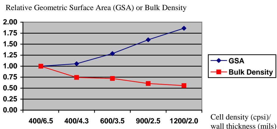
Figure 4. Relative geometric area and bulk density of ceramic substrates
