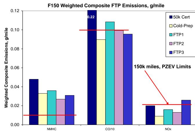
Figure 17. Weighted FTP Stock, Baseline Emissions – F-150
