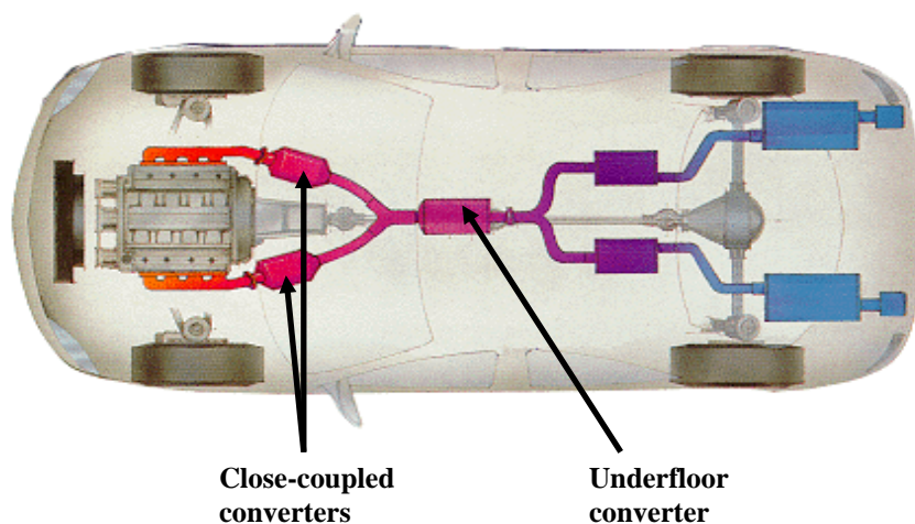
Figure 3. Exhaust system with close-coupled converters
