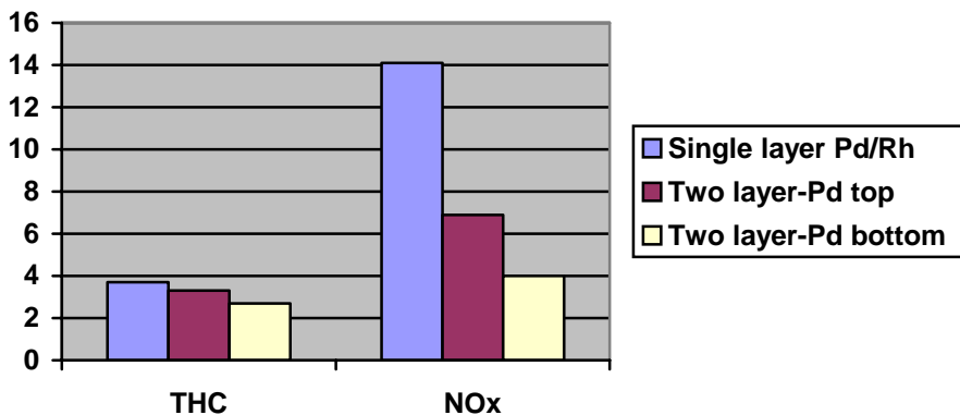
Figure 11. Impact of catalyst coating architecture (single layer vs. double layer) on total hydrocarbon (THC) and NOx performance of a Pd/Rh three-way catalyst (100 g/ft 3 total precious metal loading with Pd/Rh=5/1; 100 h aged catalyst on a 1.8 liter, 4 cylinder test vehicle; see (86) for details)
