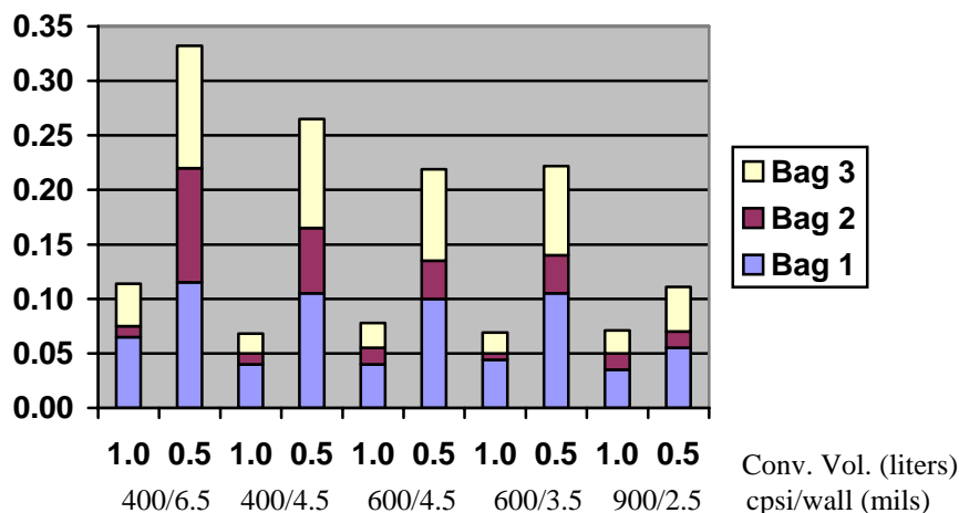
Figure 6. NO x FTP emissions for substrates with varying cell density and wall thickness [see (12) for details]
