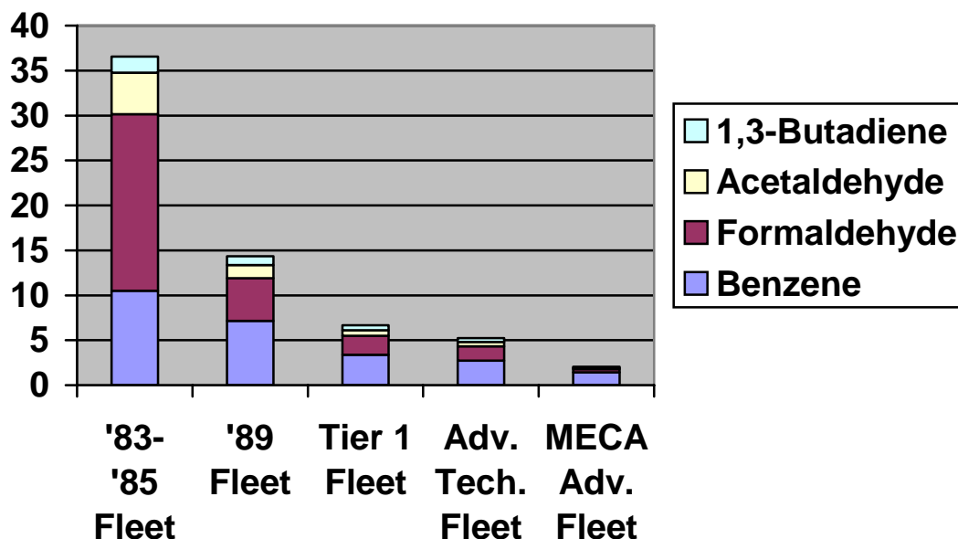
Figure 15. Toxic hydrocarbon FTP emissions from various light-duty vehicle fleets fueled with California Phase II reformulated gasoline [data for non-MECA fleets taken from U.S. Auto/Oil test programs]
