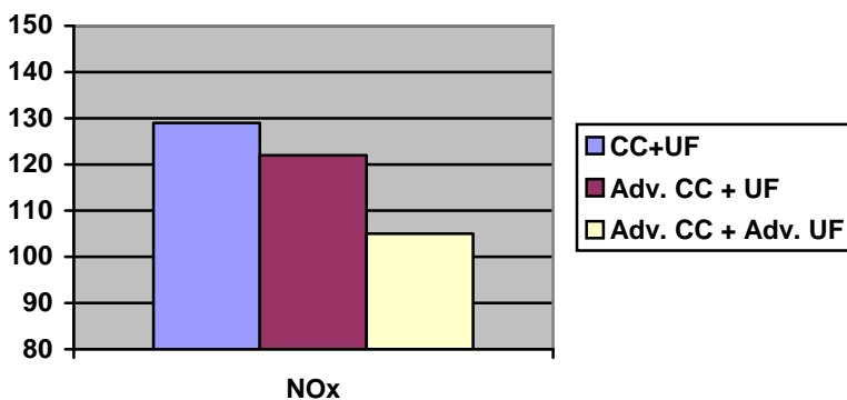
Figure 10. Impact of advanced catalyst formulations on NO x FTP emissions from a 5.3 liter, V8 test vehicle equipped with close-coupled (50 g/ft 3 Pd-only) + underfloor converters (30 g/ft 3 Pt/Rh=3/1) [see (31) for details]
