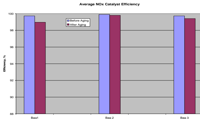
Figure 22. Denali NO x Catalyst Efficiency Comparison Before and After Advanced System Aging
