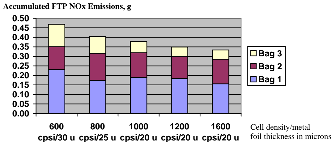
Figure 9. Accumulated FTP NO x emissions for a three-way catalyst coated on high cell density metal substrates [see (27) for details]
